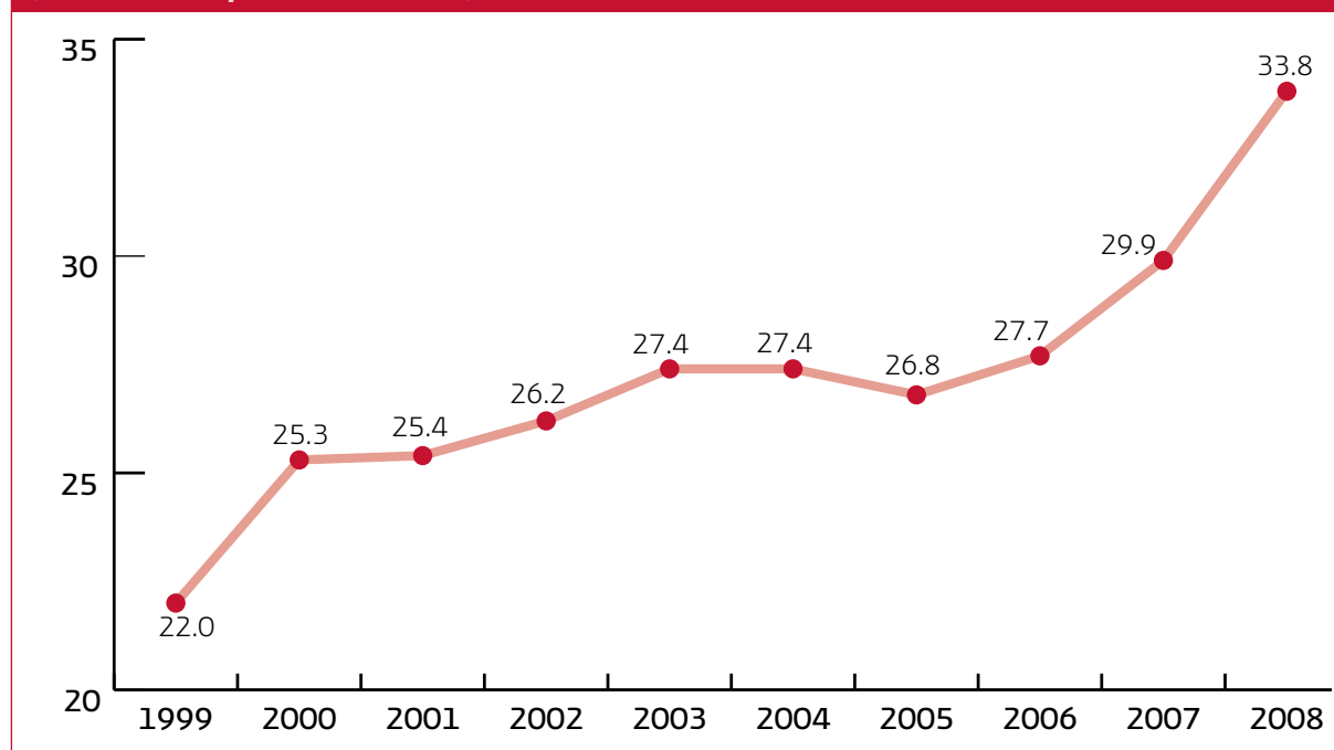
G4.14 Flow of industrial wastewater treated, annual series from 1999 to 2008 (cubic meters per second, m 3 /s)
