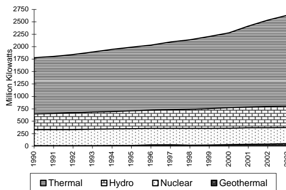
Net installed capacity of electric generating plants by type World total 1990-2003
