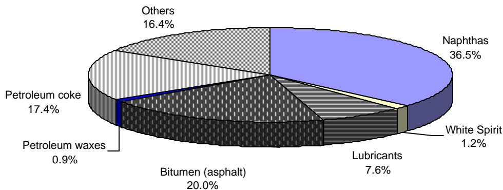
World production of non-energy products from refineries 2002
