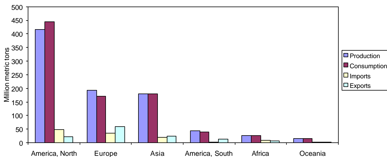
Production, trade and consumption of motor gasoline by world regions 2002
