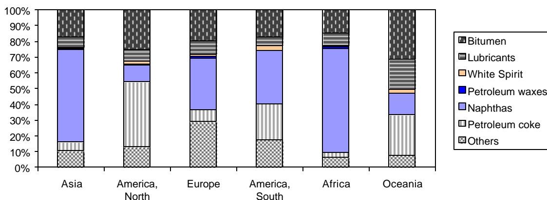
Production of non-energy products from refineries by world regions 2002
