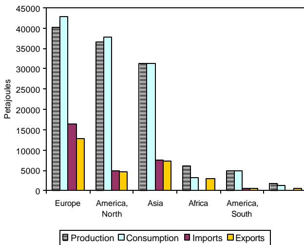
Production, trade and consumption of gases by world regions 2002
