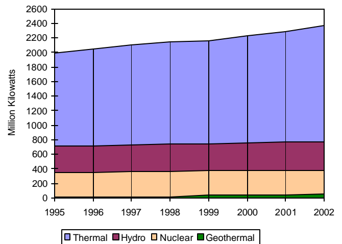
World net installed capacity of electric generating plants - by type 1995-2002
