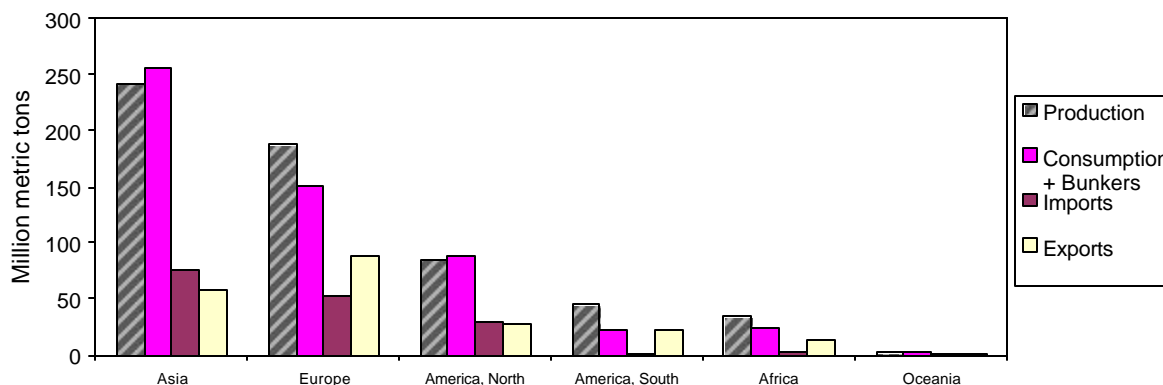
Production, trade and consumption of residual fuel oil by world regions 2002
