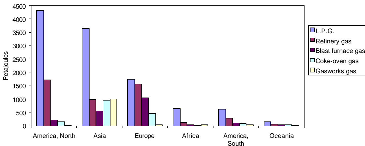
Production of other gases by type and world region 2002
