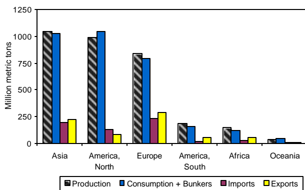
Production, trade and consumption of energy petroleum products by world regions 2002
