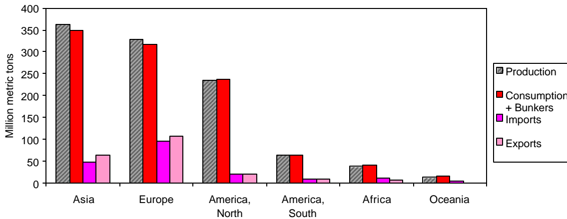
Production, trade and consumption of gas-diesel oils by world regions 2002
