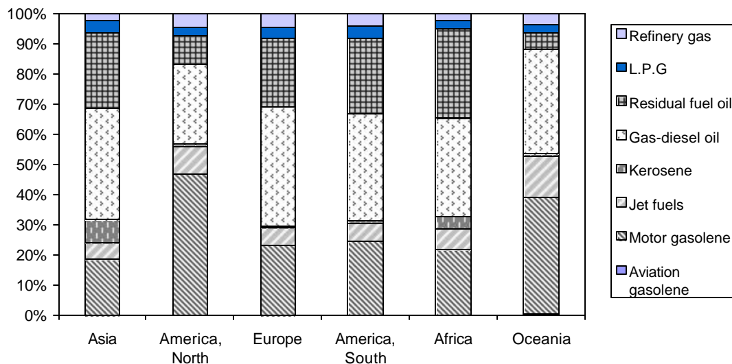
Production of energy products from refineries by world regions 2002
