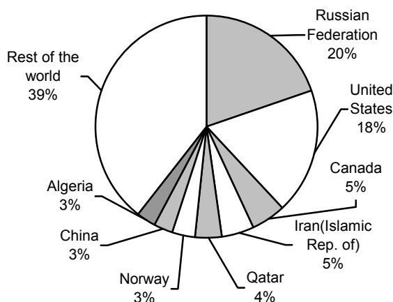
Figure 75: Major natural gas producing countries in 2010
