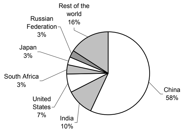
Figure 15: Major hard coal consuming countries in 2010
