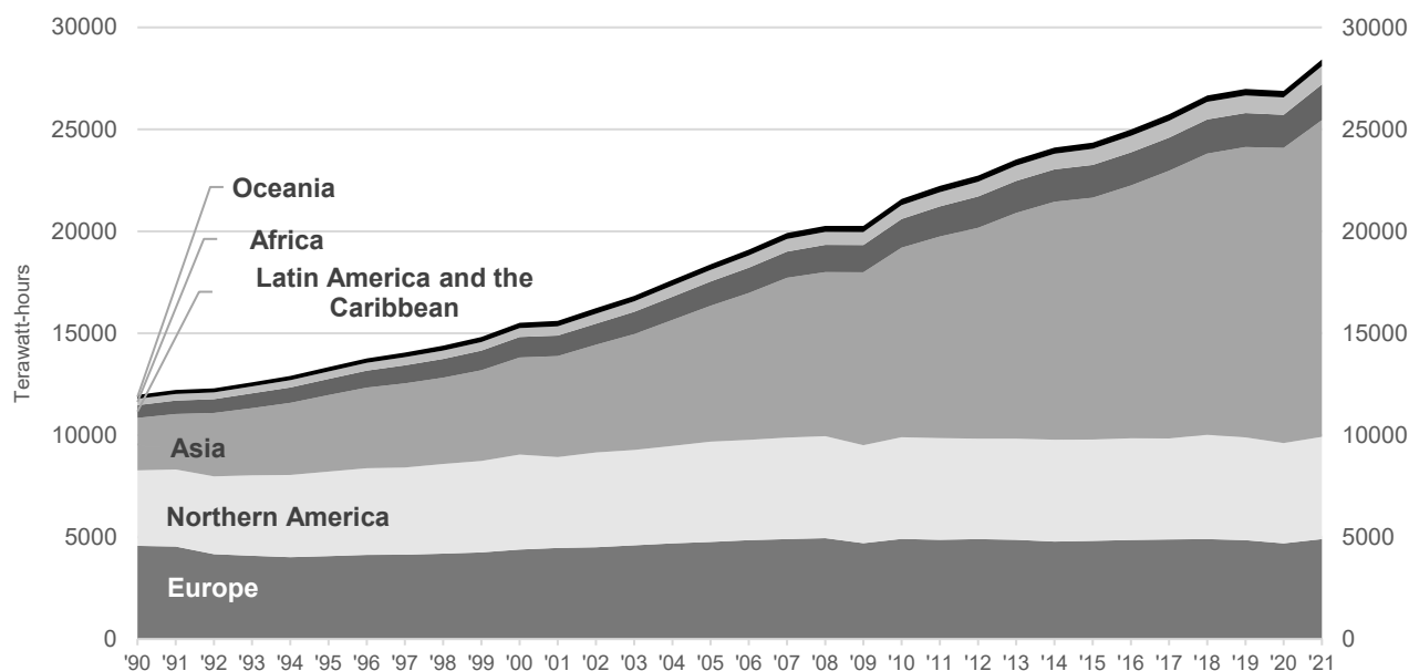
Figure 84: World electricity generation by region, 1990-2021
