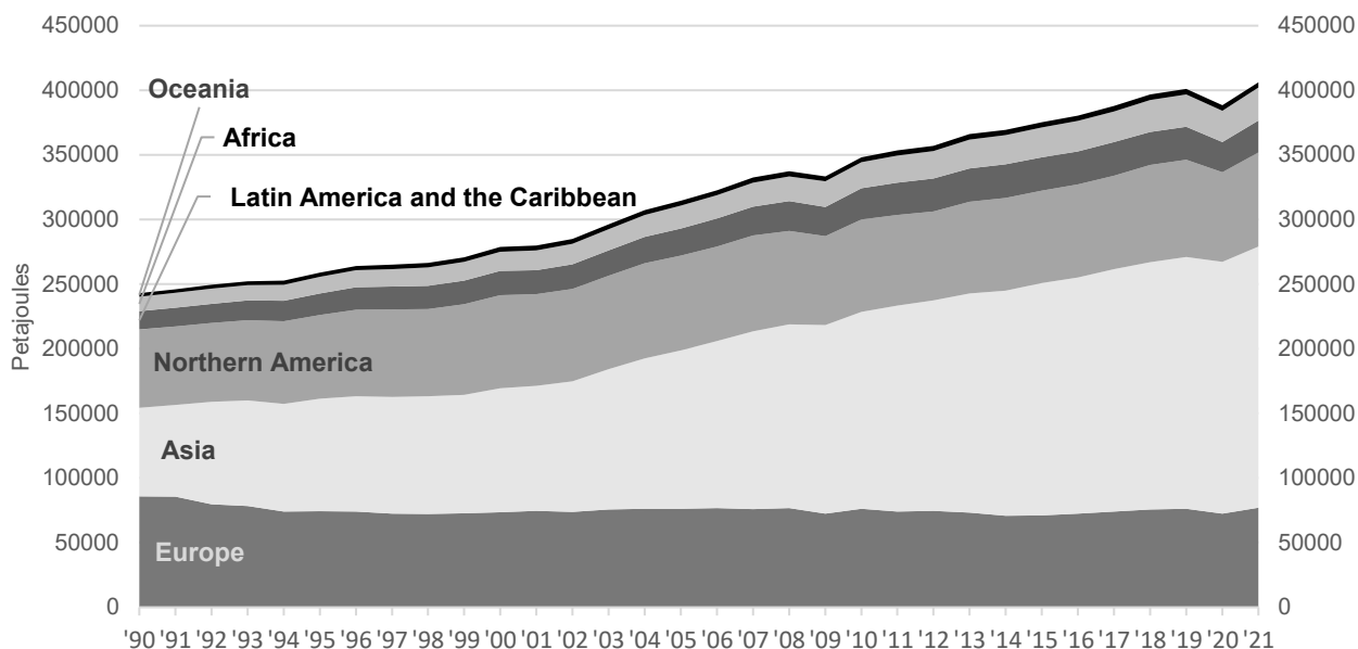
Figure 10: Total final consumption by region, 1990-2021
