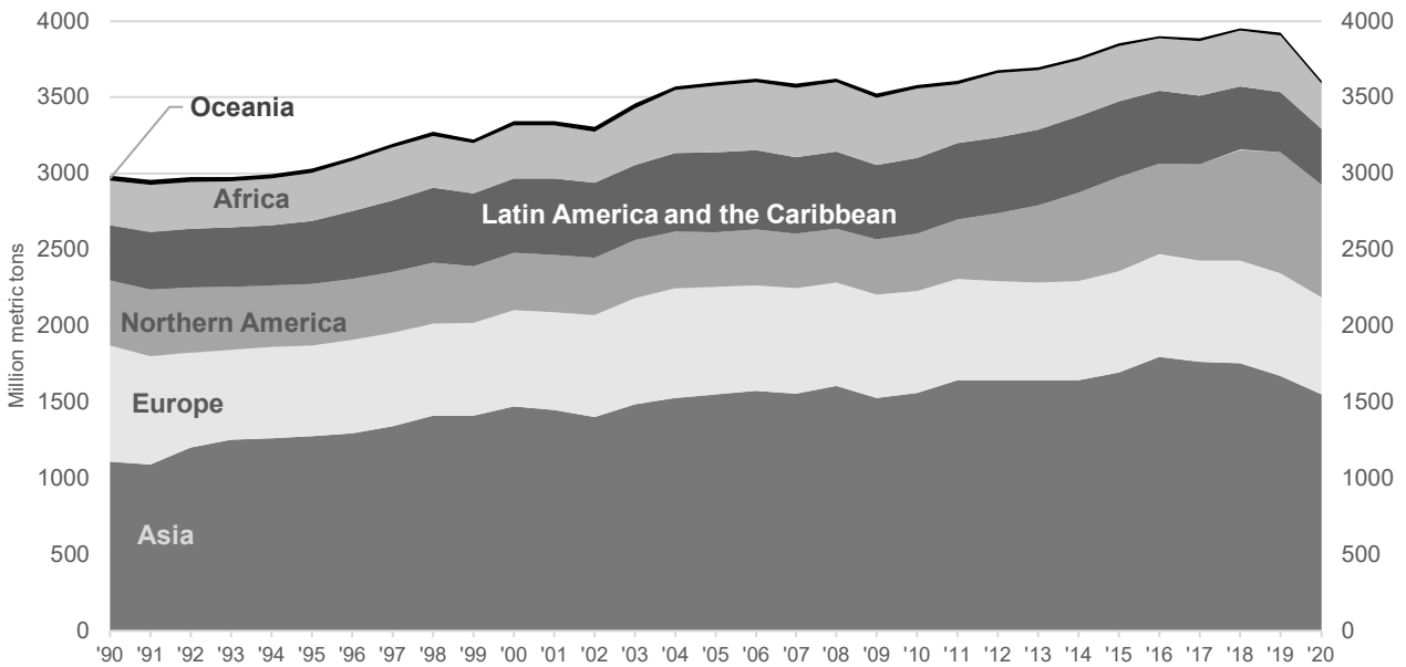
Figure 36: Production of conventional crude oil by region, 1990-2020
