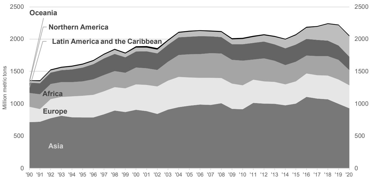
Figure 37: Exports of conventional crude oil by region, 1990-2020
