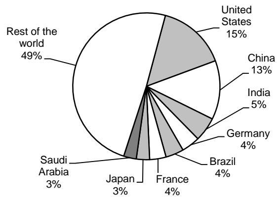
Figure 59: Major gas oil/diesel oil consuming countries, 2014
