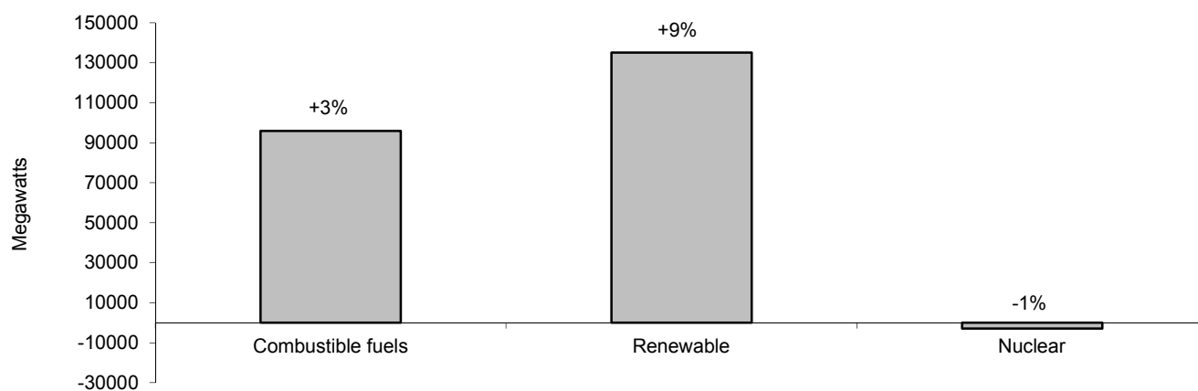
Figure 73: Change in net installed capacity of electricity generating plants*, 2012-2013
