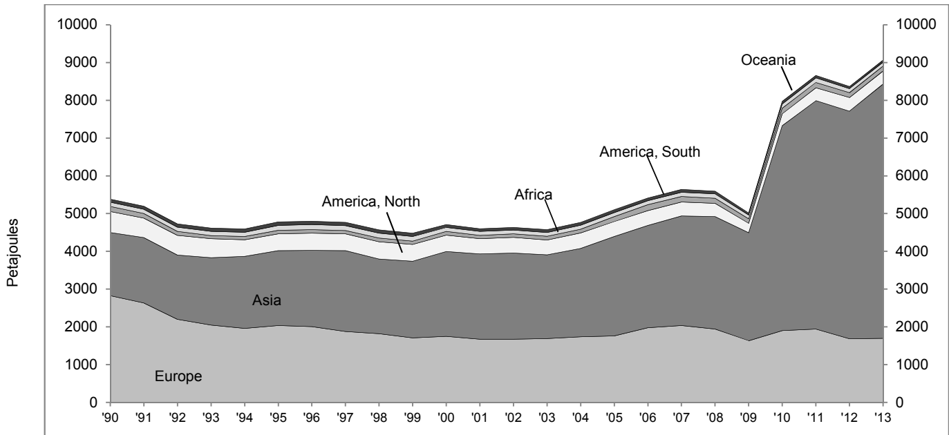
Figure 71: Production of manufactured gases by region, 1990-2013
