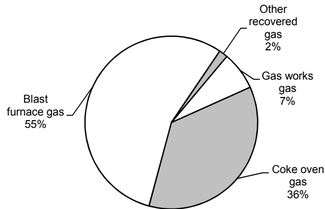
Figure 72: World production of manufactured and recovered gases by type, 2013
