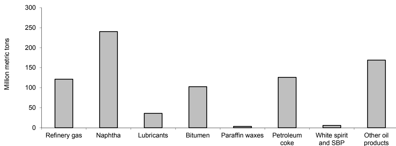
Figure 63: Production of minor oil products from refineries, 2013*
