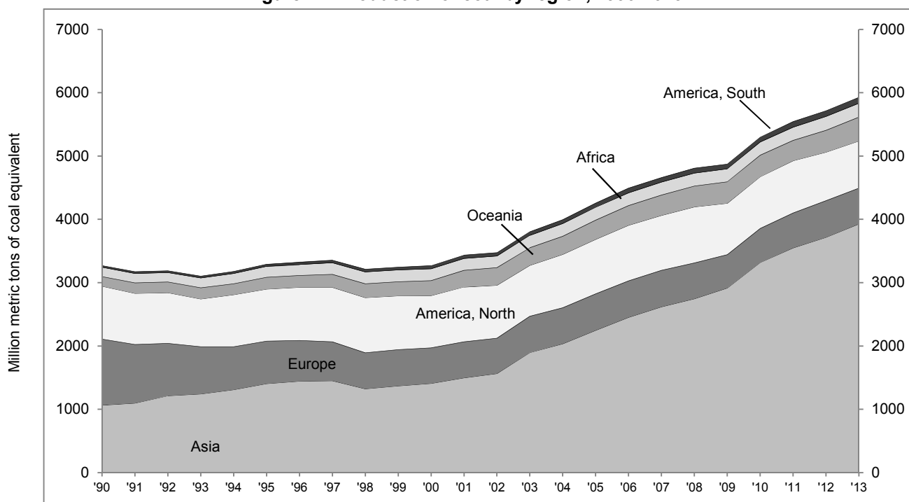
Figure 11: Production of coal by region, 1990-2013
