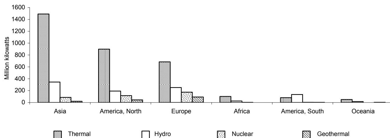
Figure 82: Net installed capacity of electric generating plants in 2009
