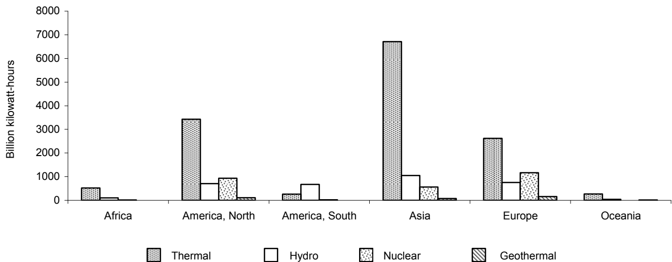
Figure 85: World electricity production, by type and region, in 2009
