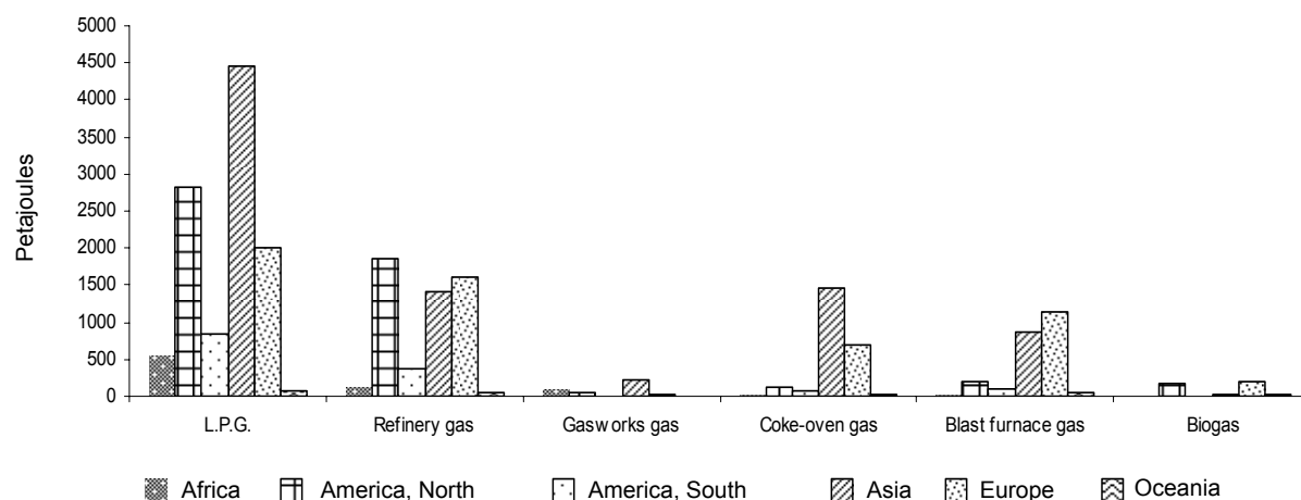
Figure 79: Production of other gases by type, by region, in 2006
