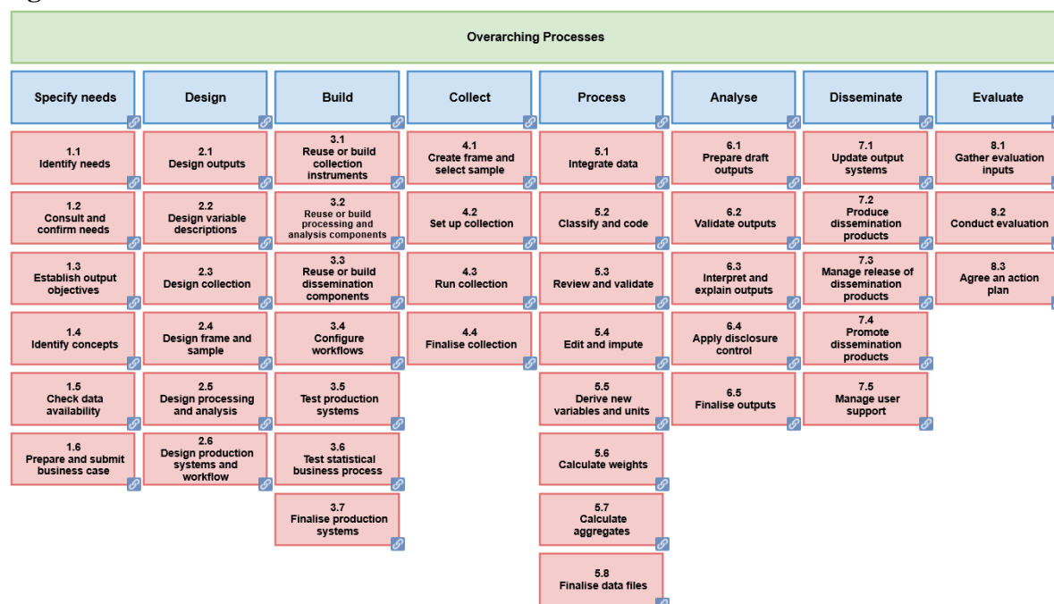
Figure 4: GSBPM
