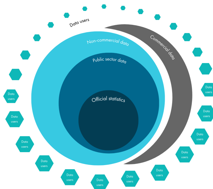
Fig. 5.1: Onion model
