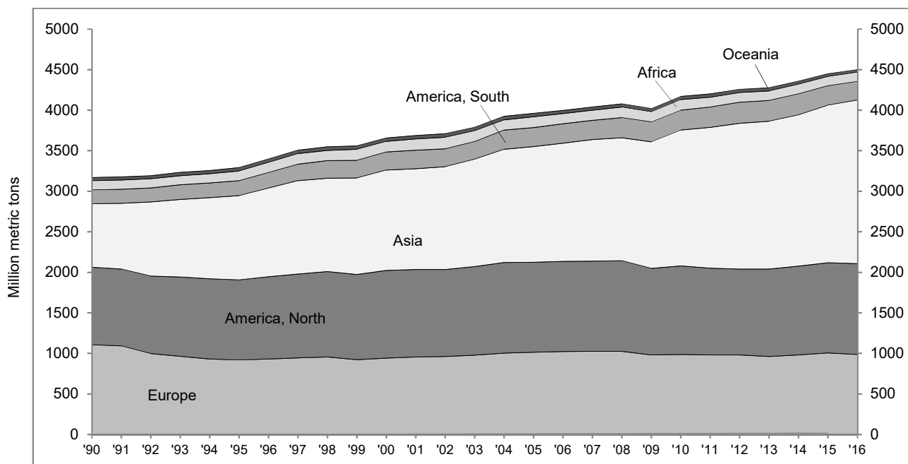
Figure 65: Production of oil products by region, 1990-2016
