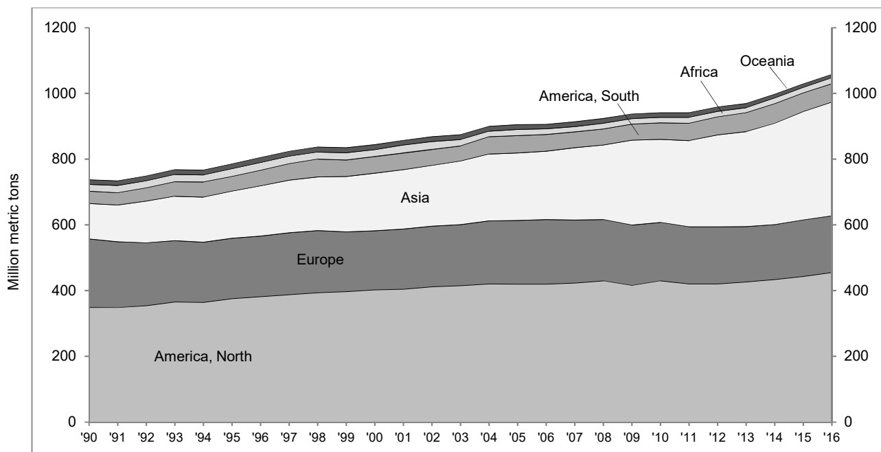
Figure 48: Production of motor gasoline by region, 1990-2016
