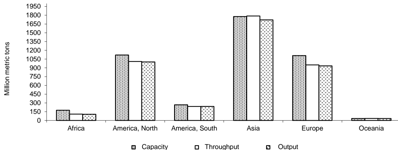
Figure 43: Refinery distillation capacity, throughput and output by region, 2014
