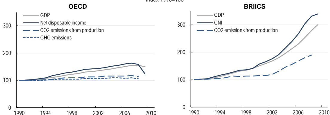
CO 2 and GHG emissions versus GDP and real income, OECD, BRIICS, 1990-2008
