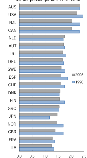
Passenger transport energy intensity
