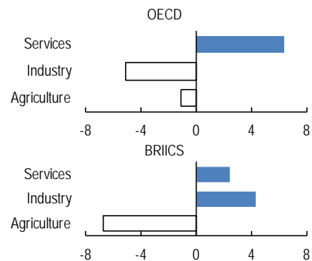
GDP structure, 1990/02-2007/09
