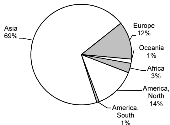
Figure 12: World solid fuel consumption, by region, in 2011
