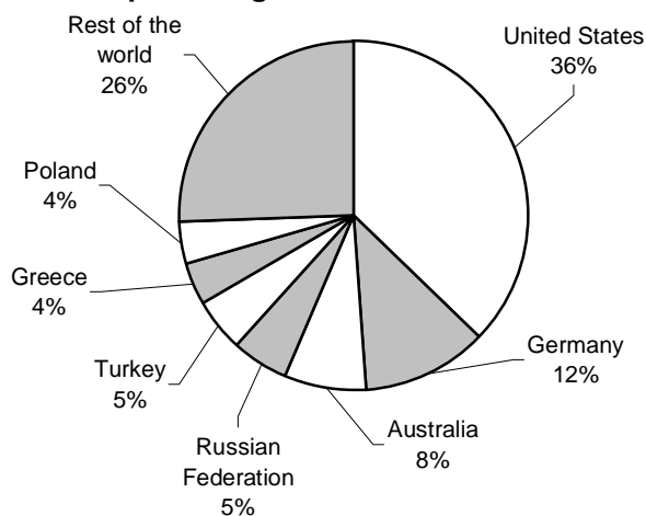
Figure 17: Major lignite and sub-bituminous coal producing countries in 2010
